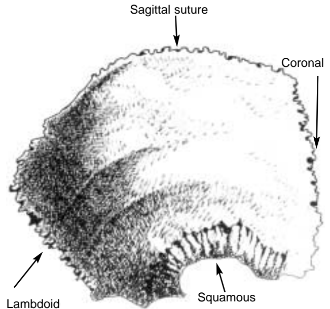
Figure 2: External view of one parietal bone. Sagittal, coronal and lambdoid sutures become dentate within first years of life and will solidify in a puzzle-like interweaving. Squamous suture is anatomically different: oblique edges of parietal and temporal bones form a 1 to 2cm zone of contact.
