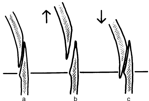
Figure 3: Junction between cranial vault and cranial base on a vertical section of a squamous suture. (a) in normal situation, oblique edge of temporal bone acts as a console, to sustain parietal bone; (b) with increasing intra-cranial pressure, parietal edge slips upward and distension occurs between 2 edges; (c) with decreasing intra-cranial pressure, parietal bone slips downward, and temporal edge becomes ridge-like.
