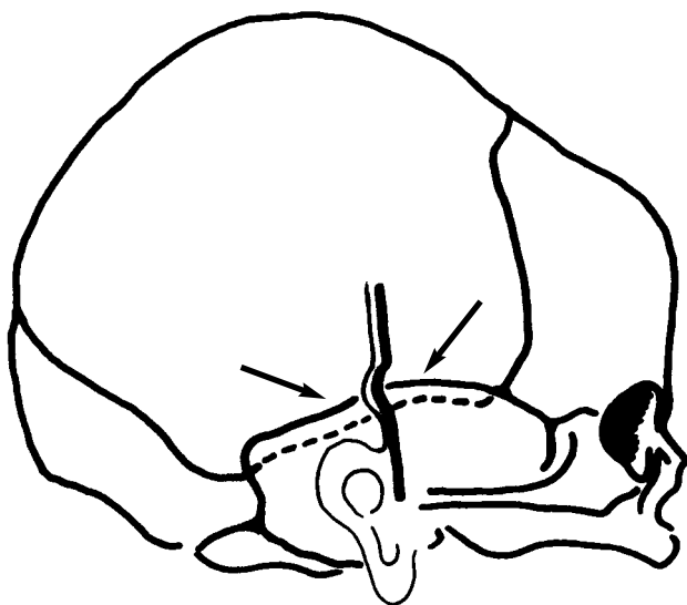
Figure 4: Squamous ridge on a profile view of skull. A prominent ridge occurs above ear when edge of temporal bone is overlapping parietal bone.
