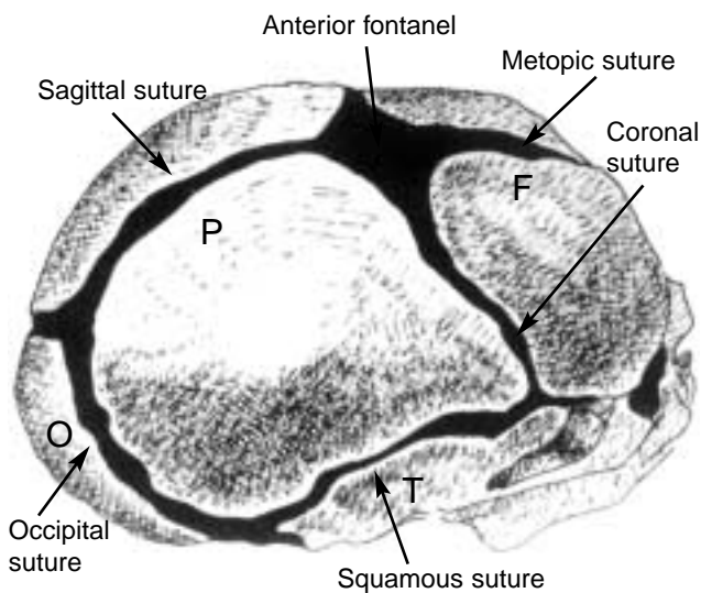
Figure 1: Skull bones, sutures and fontanel in fetus and neonate. Every suture is made of a 1 to 2mm wide membranous zone. F, frontal bone; P, parietal bone; O, occipital bone; T, temporal bone.
